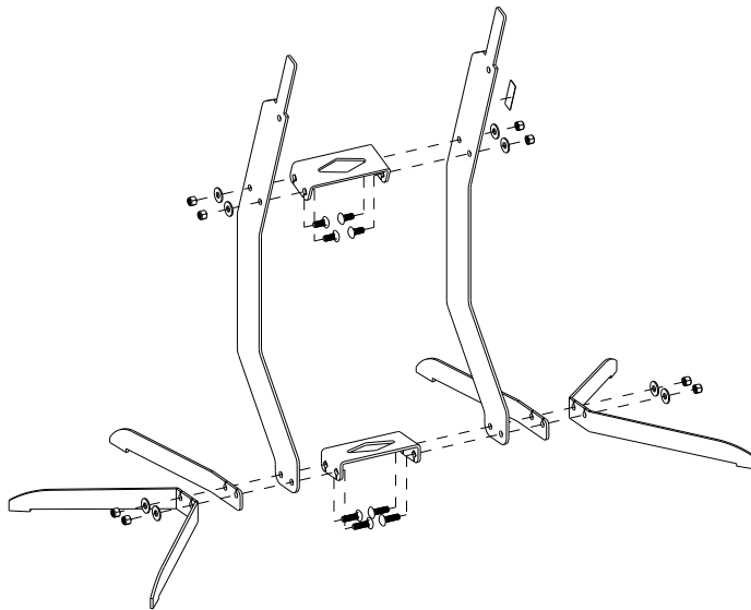
FIGURE 1: TARGET STAND ASSEMBLY
